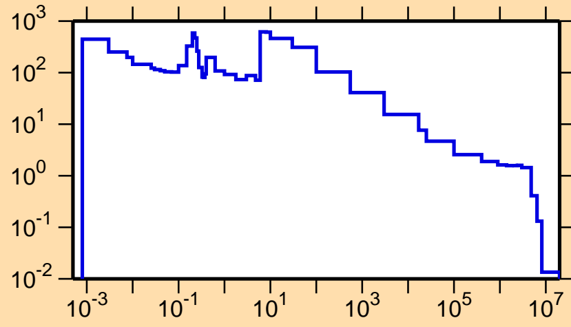
\sigma vs. E for ^{173}\text{W}(n,\gamma)
