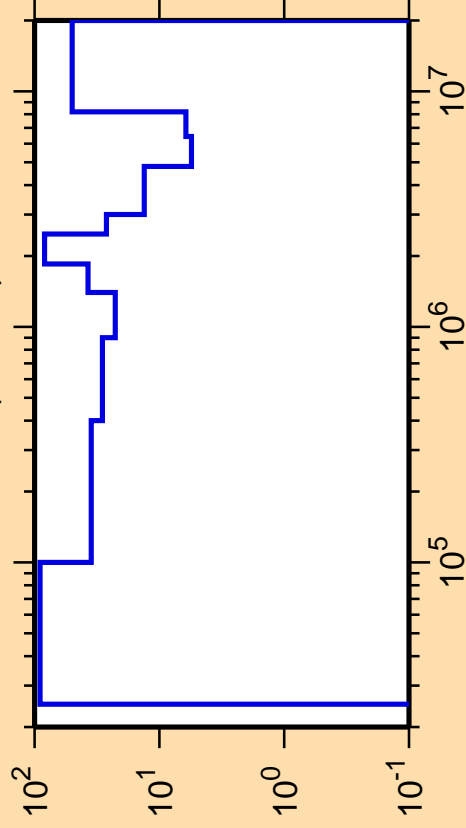
\Delta\sigma/\sigma vs. E for ^{173}\text{W}(n,\text{inel.})
