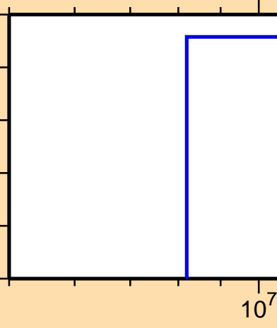
\sigma vs. E for ^{173}\text{W} (mt 11)
