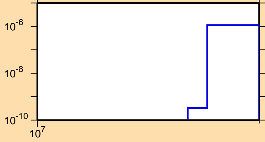
\sigma vs. E for ^{174}\text{W}(n,2np)
