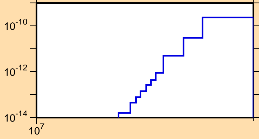
\sigma vs. E for ^{174}\text{W}(\text{mt117})
