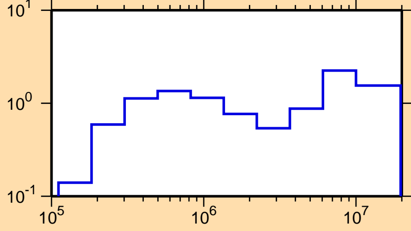
\sigma vs. E for ^{174}\text{W}(n,\text{inel.})
