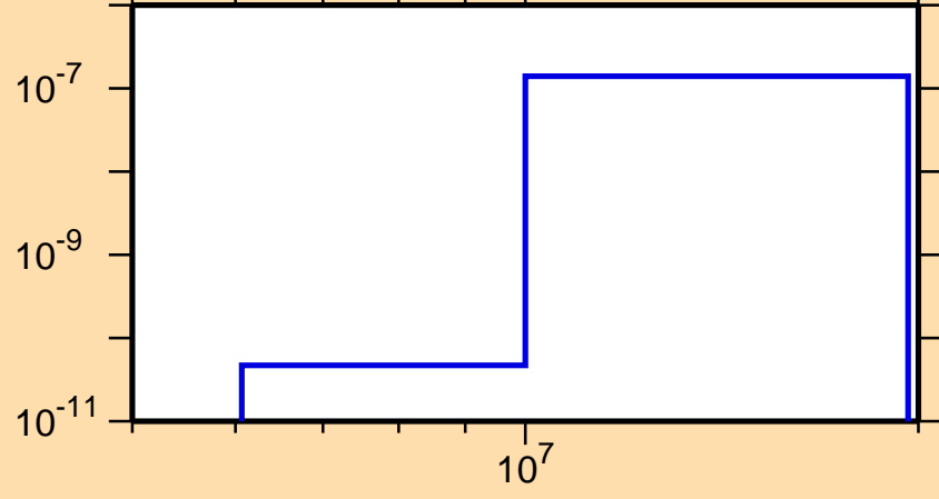
\sigma vs. E for ^{174}\text{W}(n,p\alpha)
