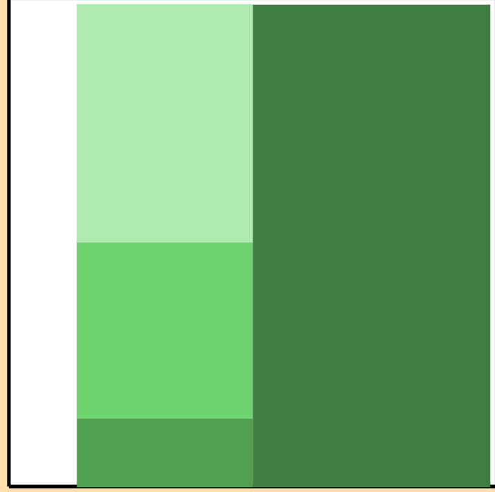
\Delta\sigma/\sigma vs. E for ^{174}\text{W}(n,2n)
