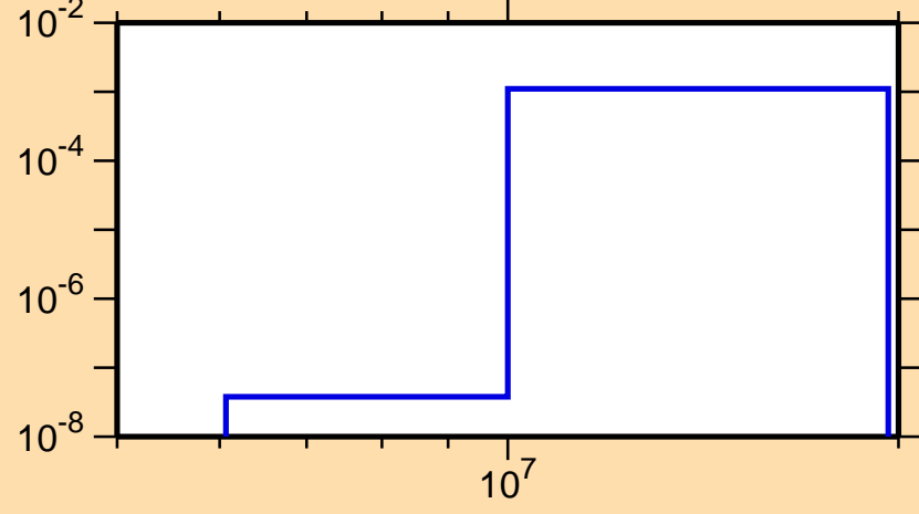
\sigma vs. E for ^{174}\text{W}(n,d)
