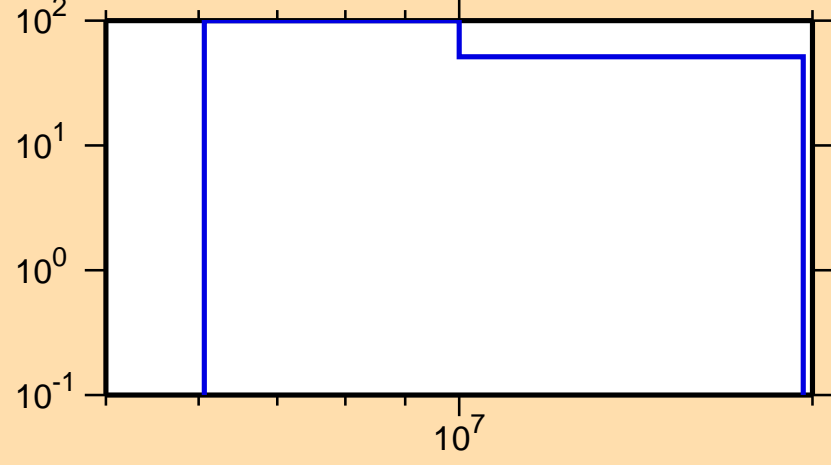
\Delta\sigma/\sigma vs. E for ^{174}\text{W}(n,2n)
