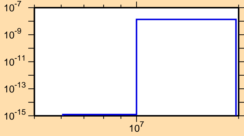
\sigma vs. E for ^{174}\text{W}(n,\text{He3})
