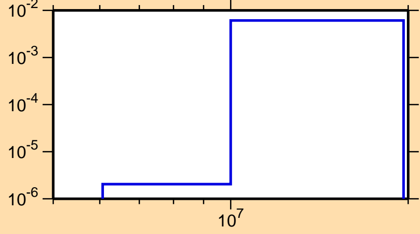
\sigma vs. E for ^{174}\text{W}(n,np)
