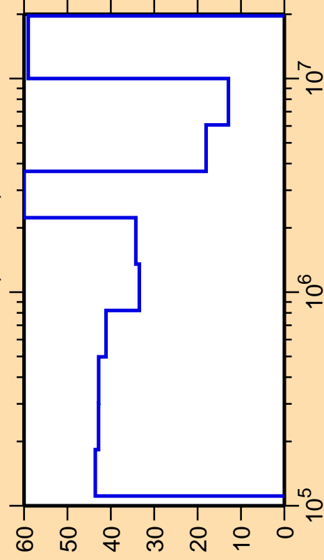
\Delta\sigma/\sigma vs. E for ^{174}\text{W}(n,\text{inel.})
