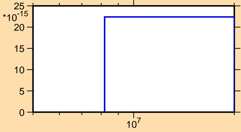
\sigma vs. E for ^{174}\text{W}(n,\text{pt})
