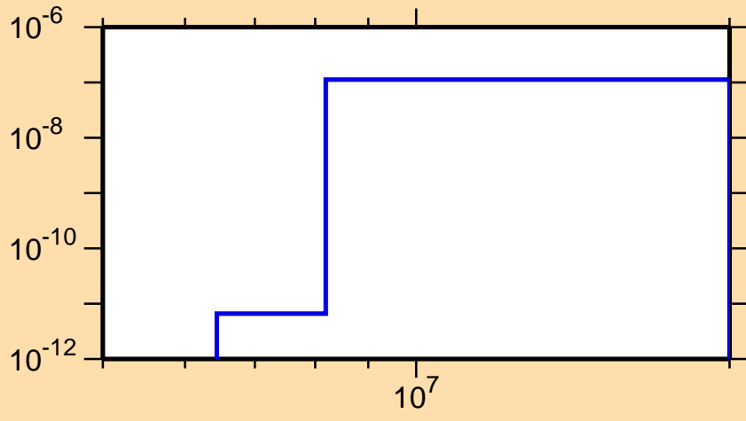
\sigma vs. E for ^{174}\text{W}(n,p\alpha)
