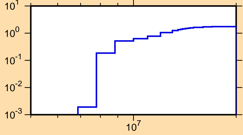
\sigma vs. E for ^{175}\text{W}(n,2n)
