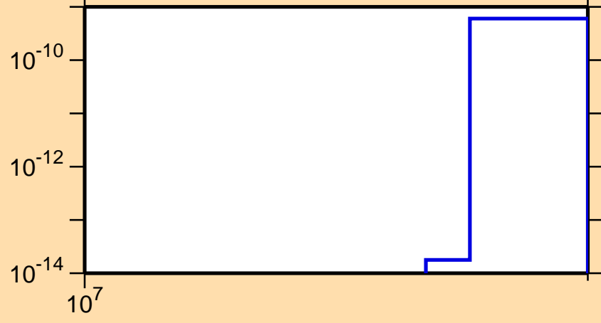
\sigma vs. E for ^{175}\text{W}(n,nt)
