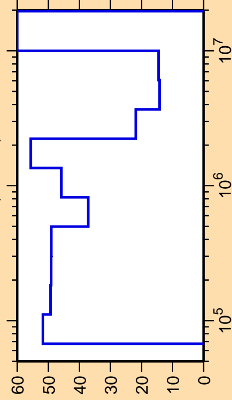
\Delta\sigma/\sigma vs. E for ^{175}\text{W}(n,\text{inel.})
