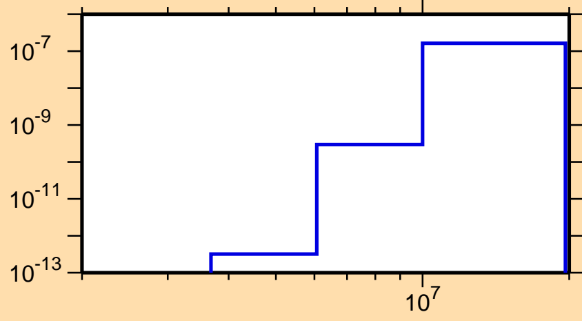
\sigma vs. E for ^{175}\text{W}(n,p\alpha)
