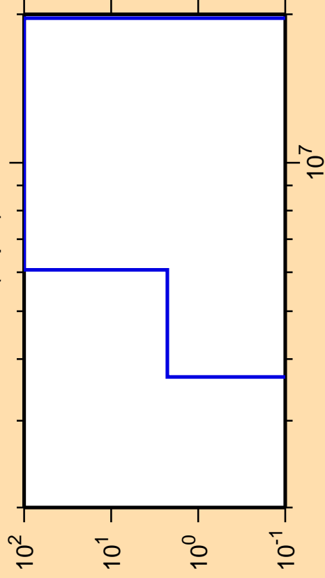
\Delta\sigma/\sigma vs. E for ^{175}\text{W}(n,p\alpha)
