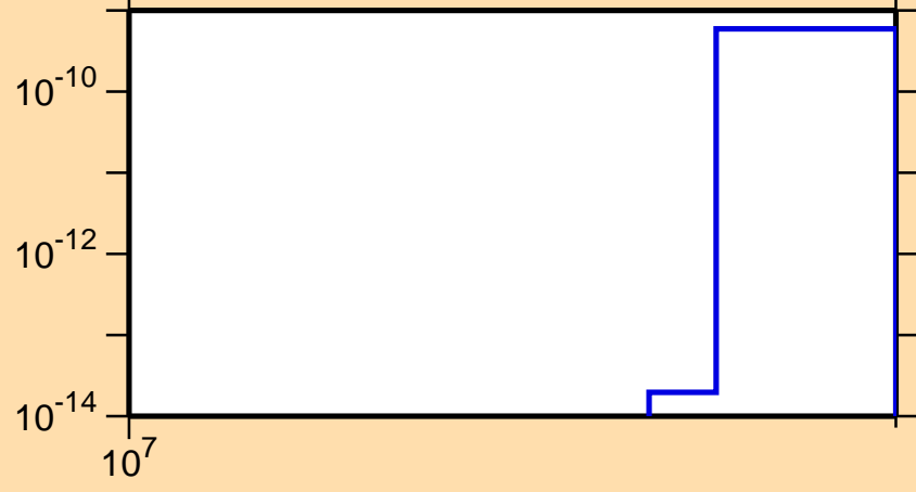
\sigma vs. E for ^{176}\text{W}(n,nt)
