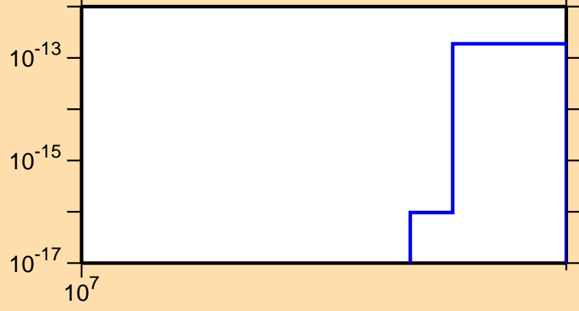
\sigma vs. E for ^{176}\text{W}(n,\text{pt})
