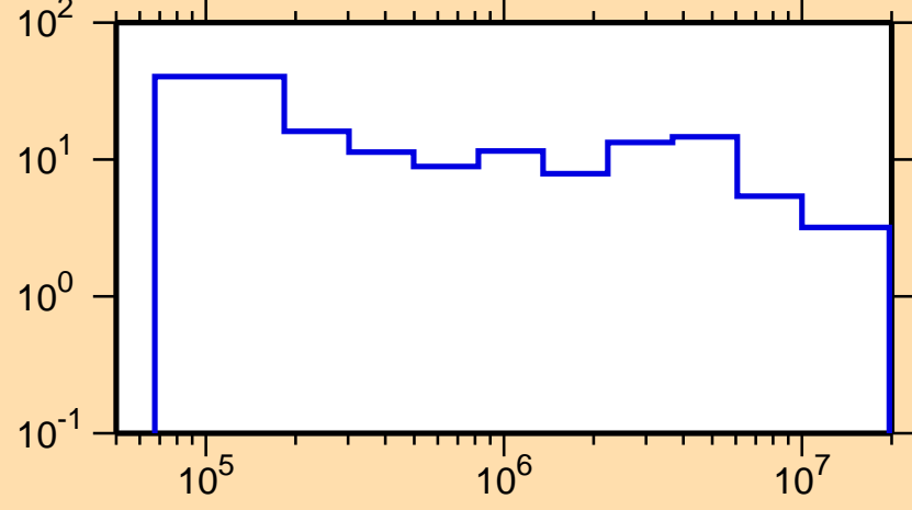
\Delta\sigma/\sigma vs. E for ^{176}\text{W}(n,\text{tot.})
