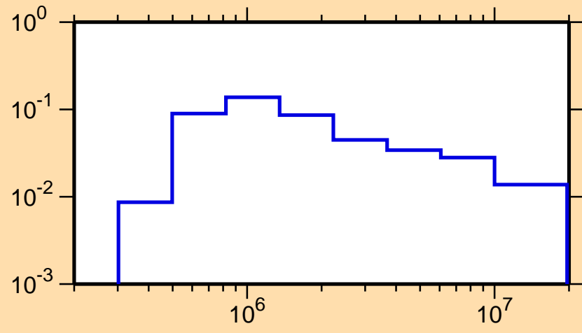
\sigma vs. E for ^{176}\text{W}(n,n_2)
