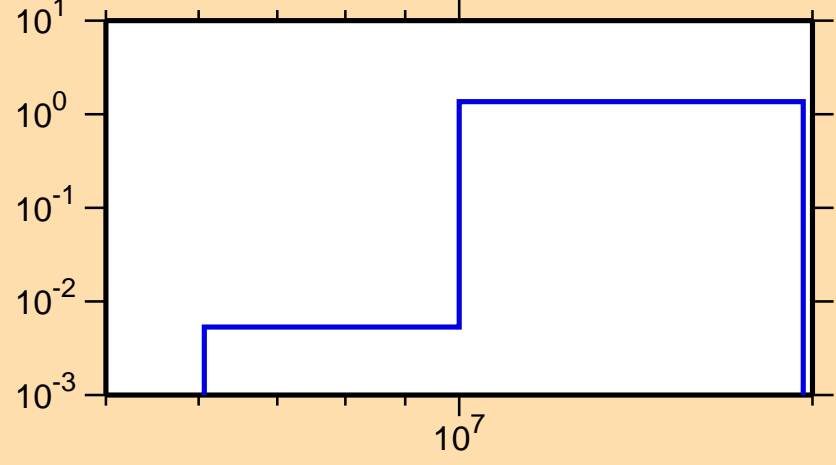
\sigma vs. E for ^{176}\text{W}(n,2n)
