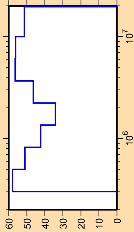
\Delta\sigma/\sigma vs. E for ^{176}\text{W}(n,n_2)
