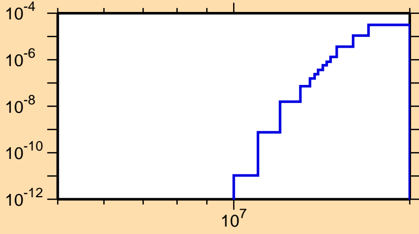
\sigma vs. E for ^{177}\text{W}(n,2n\alpha)
