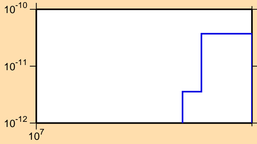
\sigma vs. E for ^{177}\text{W} (mt 45)
