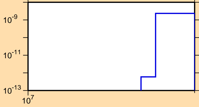
\sigma vs. E for ^{177}\text{W}(n,nt)
