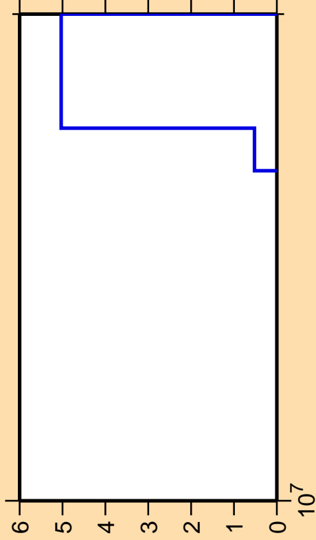
\Delta\sigma/\sigma vs. E for ^{179}\text{W}(\text{mt117})
