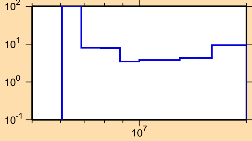
\Delta\sigma/\sigma vs. E for ^{179}\text{W}(n,2n)
