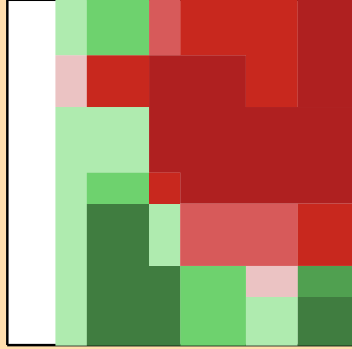
\Delta\sigma/\sigma vs. E for ^{179}\text{W}(n,2n)
