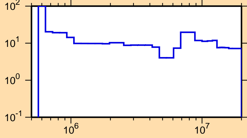
\Delta\sigma/\sigma vs. E for ^{179}\text{W}(n,n\text{cont.})
