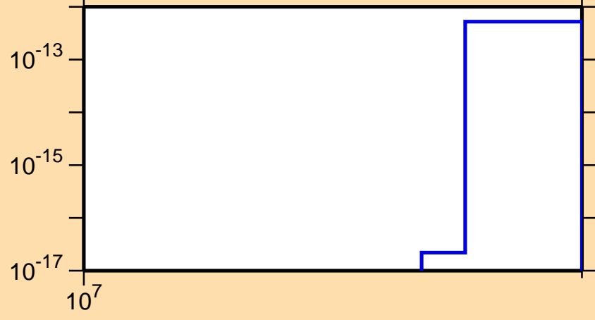
\sigma vs. E for ^{179}\text{W}(n,3n\alpha)
