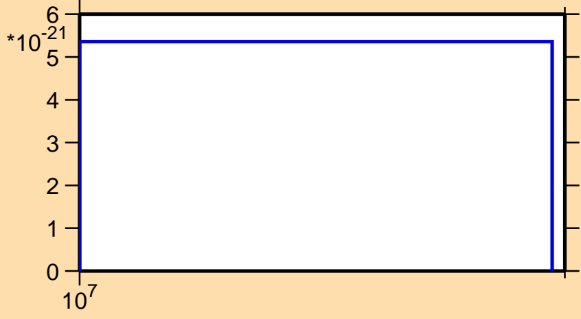
\sigma vs. E for ^{179}\text{W} (mt 11)
