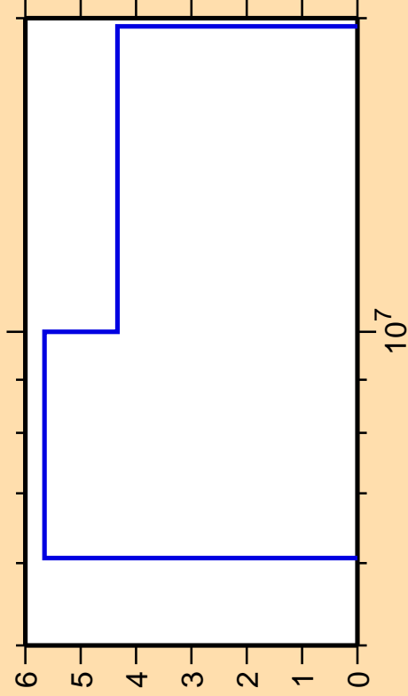
\Delta\sigma/\sigma vs. E for ^{179}\text{W}(n,2n)
