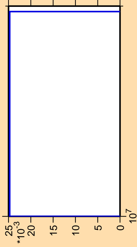
\Delta\sigma/\sigma vs. E for ^{179}\text{W}(n,\text{pt})
