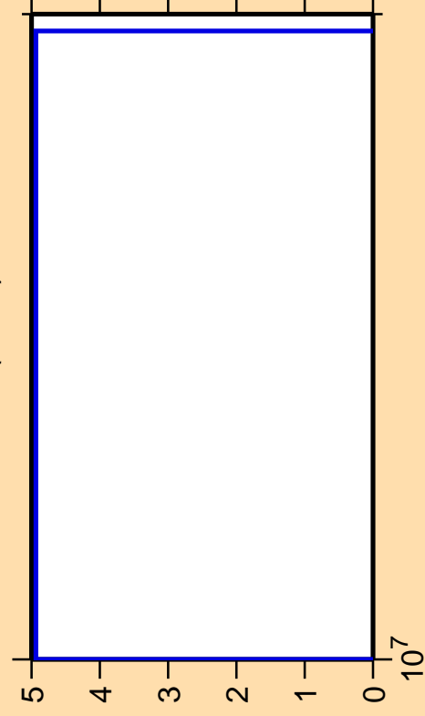
\Delta\sigma/\sigma vs. E for ^{179}\text{W}(n,3n)
