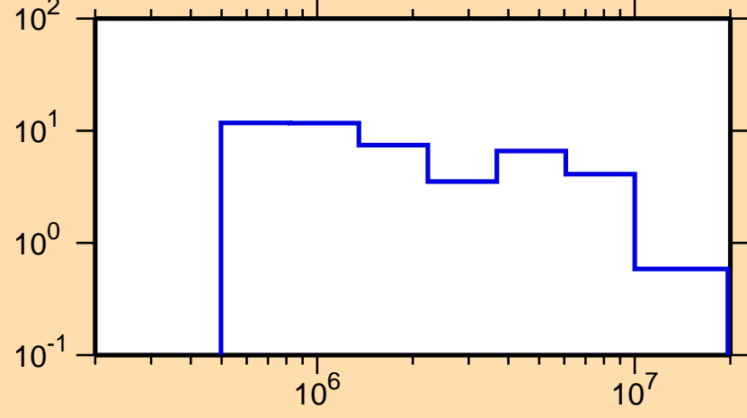
\Delta\sigma/\sigma vs. E for ^{179}\text{W}(n,\text{tot.})
