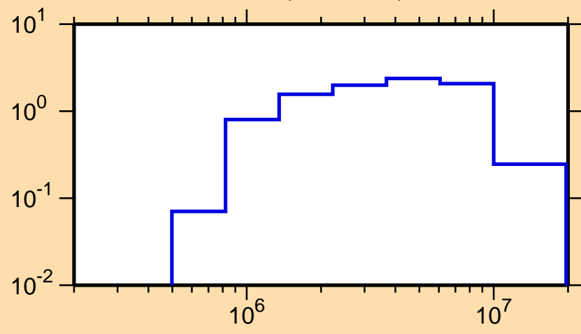
\sigma vs. E for ^{179}\text{W}(n,n\text{cont.})
