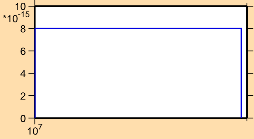
\sigma vs. E for ^{179}\text{W}(n,\text{pt})
