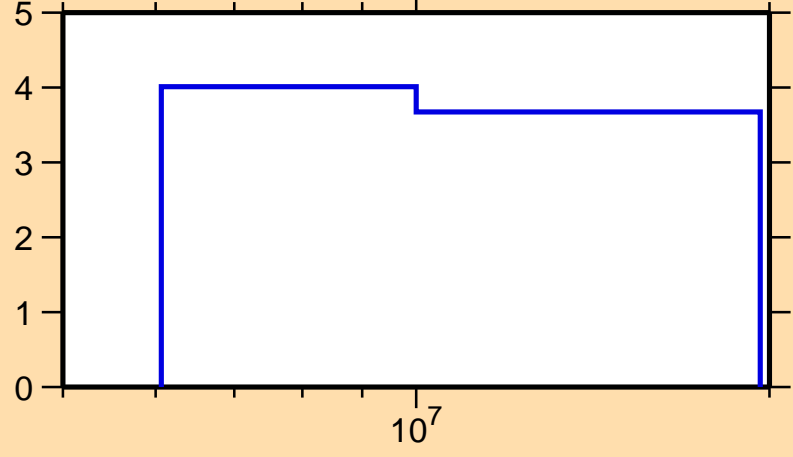
\Delta\sigma/\sigma vs. E for ^{179}\text{W}(n,\text{nonel.})
