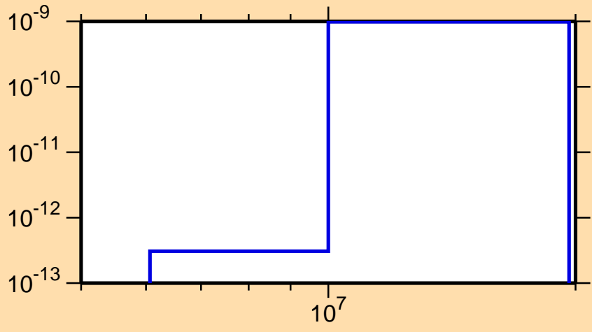
\sigma vs. E for ^{179}\text{W}(n,p\alpha)
