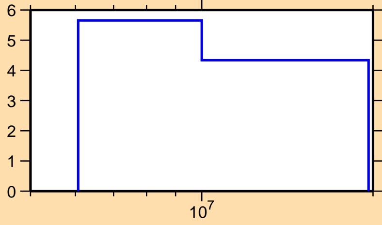
\Delta\sigma/\sigma vs. E for ^{179}\text{W}(n,2n)
