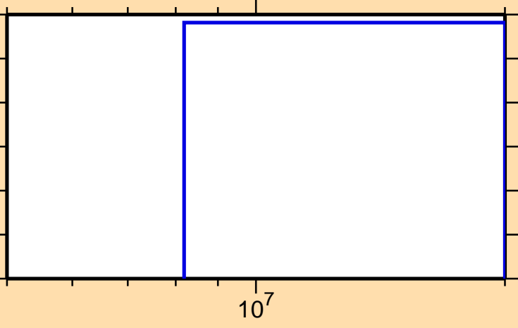
\sigma vs. E for ^{179}\text{W}(n,t)
