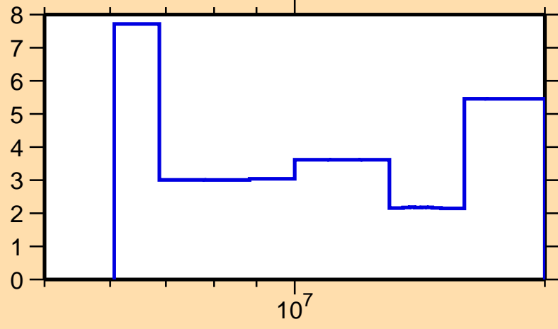
\Delta\sigma/\sigma vs. E for ^{181}\text{W}(n,\text{tot.})
