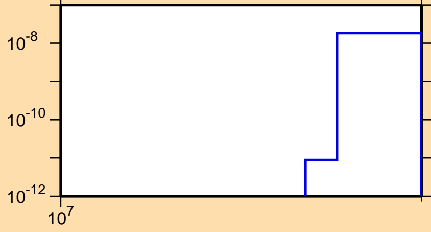
\sigma vs. E for ^{181}\text{W}(n,nt)
