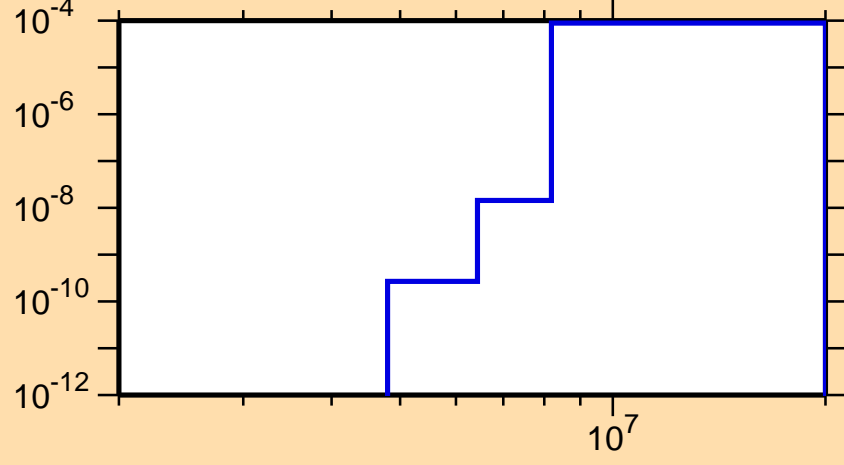
\sigma vs. E for ^{181}\text{W}(n,n\alpha)
