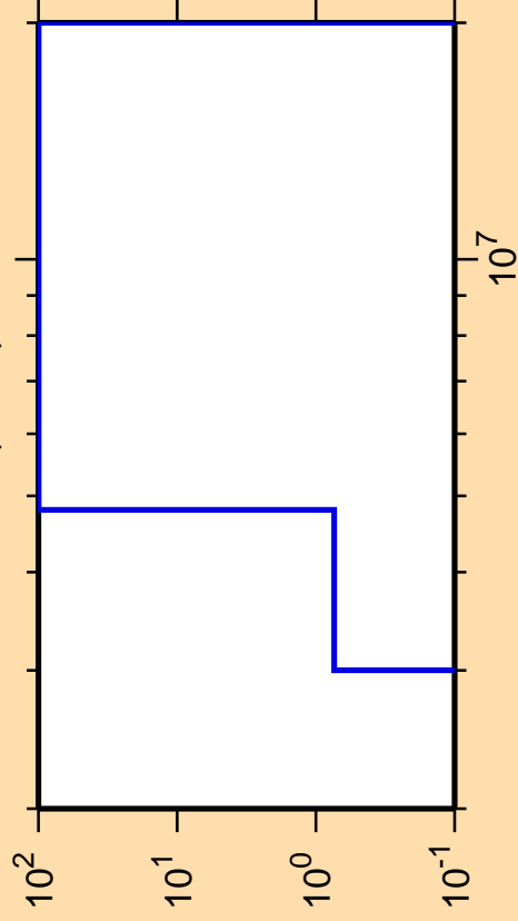
\Delta\sigma/\sigma vs. E for ^{181}\text{W}(n,n\alpha)
