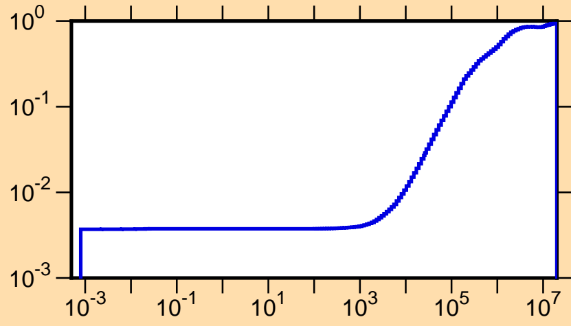
\mu vs. E for ^{182}\text{W}(\text{mt251})
