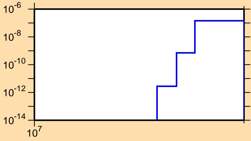
\sigma vs. E for ^{182}\text{W}(n,\text{nd})
