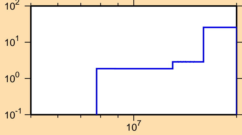
\Delta\sigma/\sigma vs. E for ^{182}\text{W}(n,2n)
