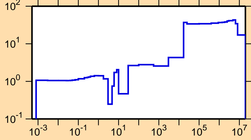
\Delta\sigma/\sigma vs. E for ^{182}\text{W}(n,\text{tot.})
