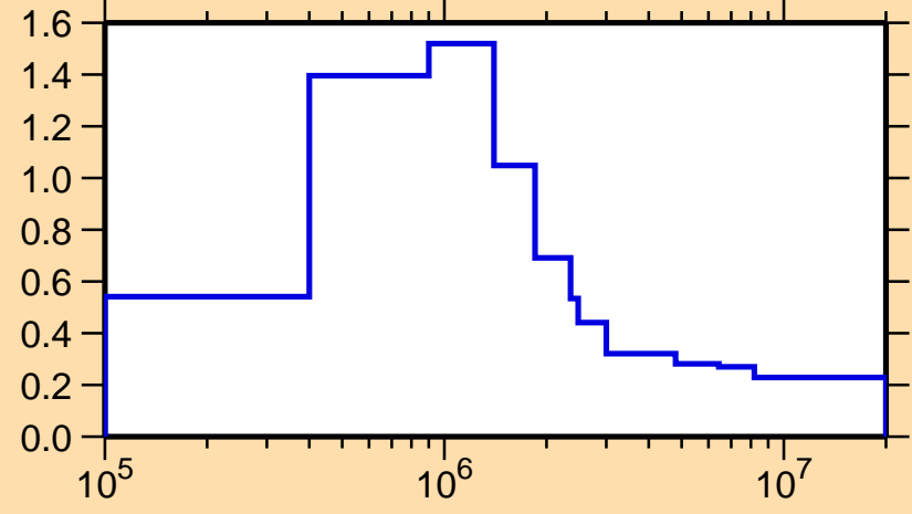
\sigma vs. E for ^{182}\text{W}(n,n_1)
