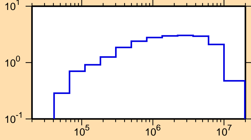
\sigma vs. E for ^{183}\text{W}(n,\text{inel.})
