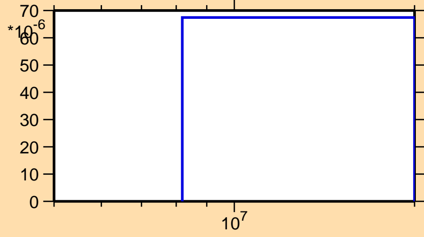
\sigma vs. E for ^{183}\text{W}(n,t)
