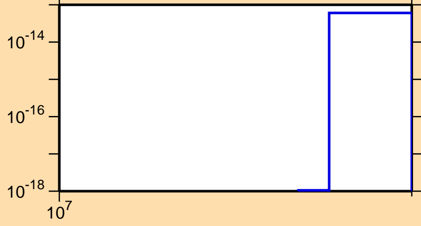
\sigma vs. E for ^{185}\text{W}(n,3n\alpha)
