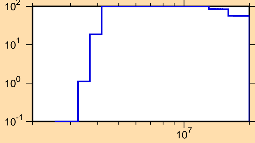
\Delta\sigma/\sigma vs. E for ^{185}\text{W}(n,p)
