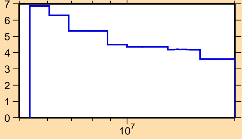
\Delta\sigma/\sigma vs. E for ^{185}\text{W}(n,\text{nonel.})
