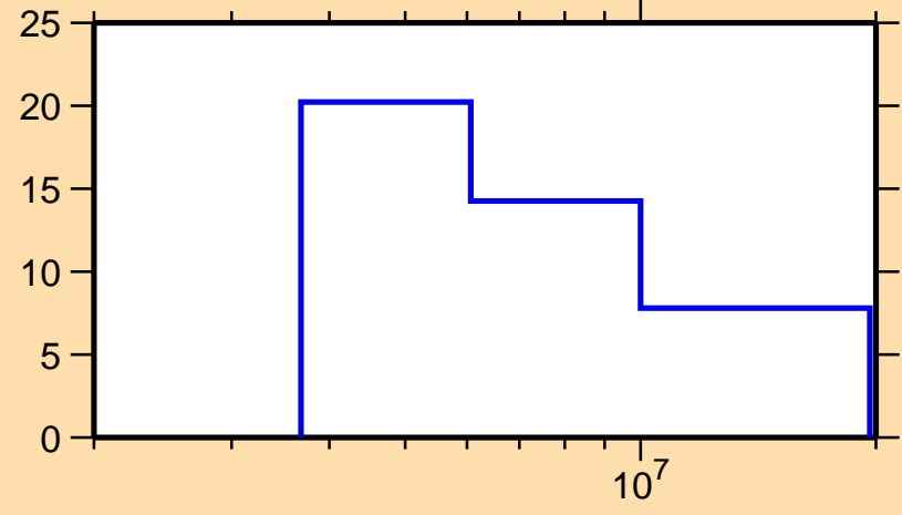
\Delta\sigma/\sigma vs. E for ^{185}\text{W}(n,el.)
