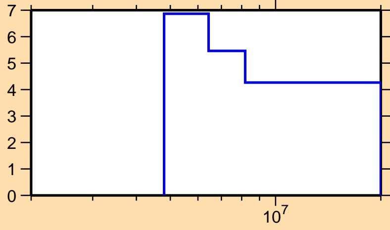
\Delta\sigma/\sigma vs. E for ^{185}\text{W}(n,\text{nonel.})
