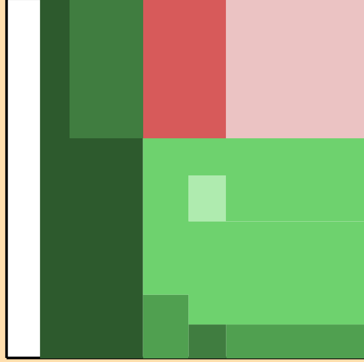
\Delta\sigma/\sigma vs. E for ^{185}\text{W}(n,p)
