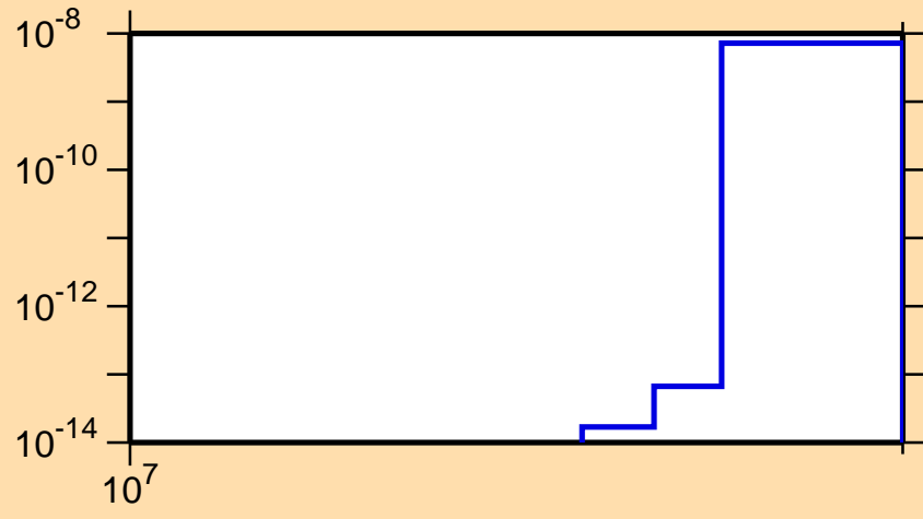
\sigma vs. E for ^{186}\text{W}(n,2np)
