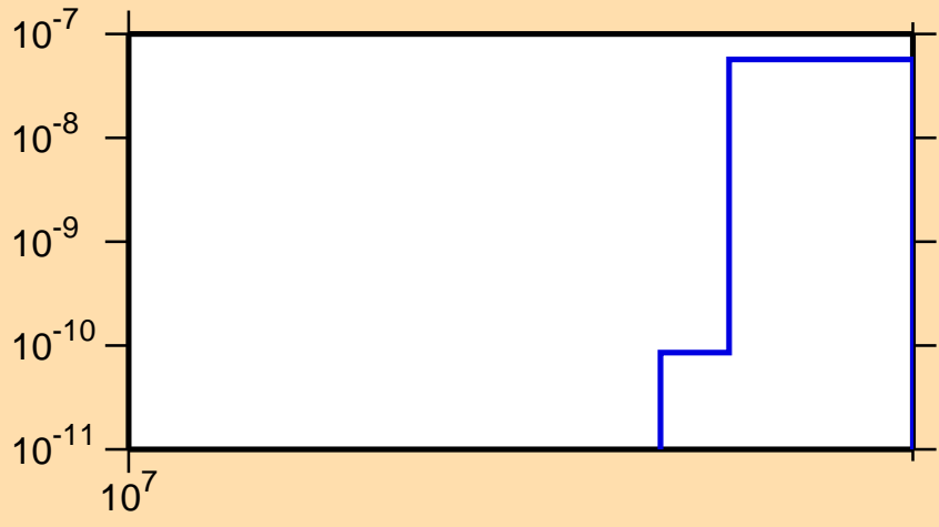
\sigma vs. E for ^{186}\text{W}(n,\text{nd})
