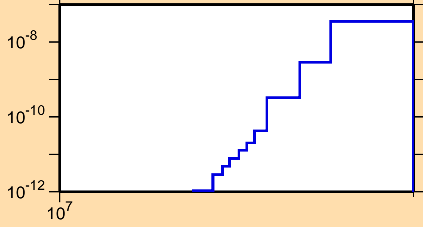
\sigma vs. E for ^{186}\text{W}(n,2n\alpha)
