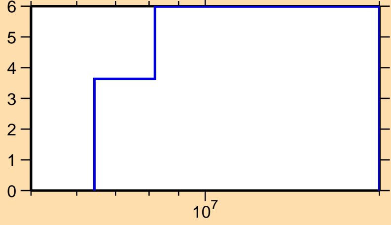
\Delta\sigma/\sigma vs. E for ^{186}\text{W}(n,\text{el.})
