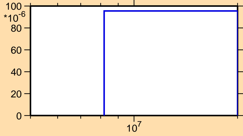
\sigma vs. E for ^{186}\text{W}(n,d)
