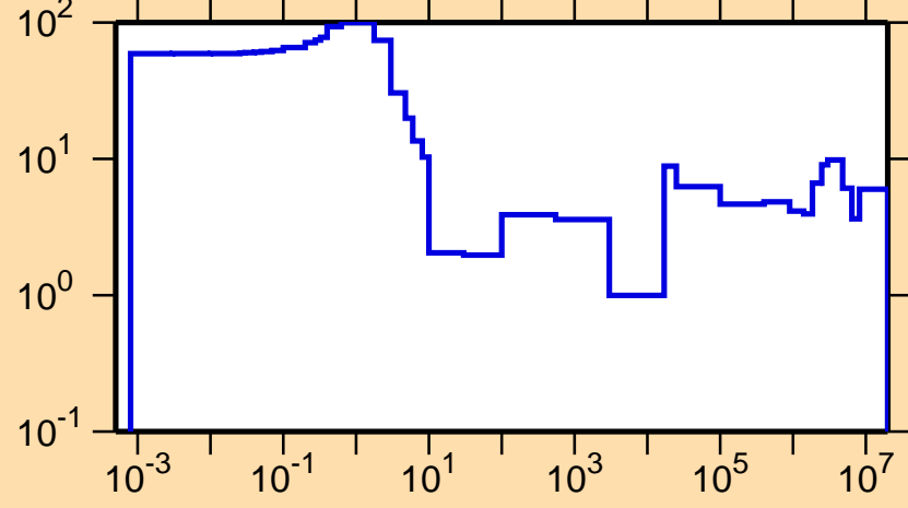
\Delta\sigma/\sigma vs. E for ^{186}\text{W}(n,\text{el.})
