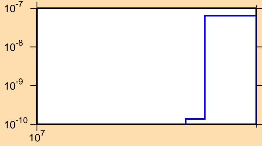
\sigma vs. E for ^{187}\text{W}(n,nt)
