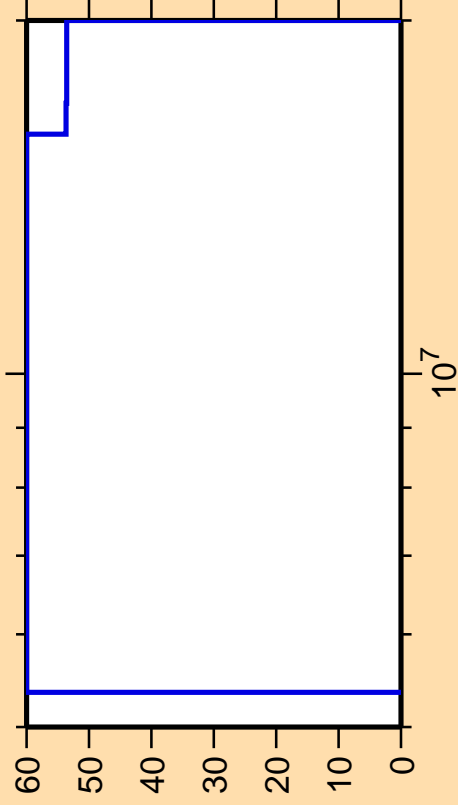
\Delta\sigma/\sigma vs. E for ^{187}\text{W}(n,\alpha)
