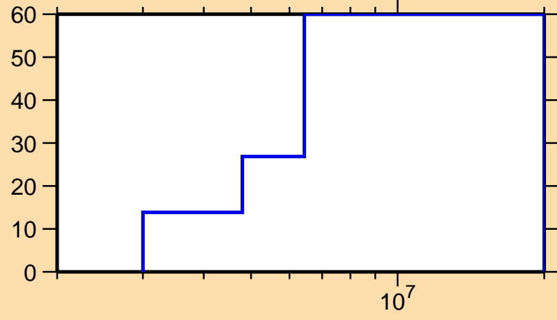
\Delta\sigma/\sigma vs. E for ^{187}\text{W}(n,ncont.)
