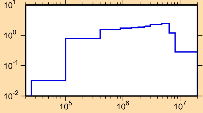
\sigma vs. E for ^{187}\text{W}(n,\text{inel.})
