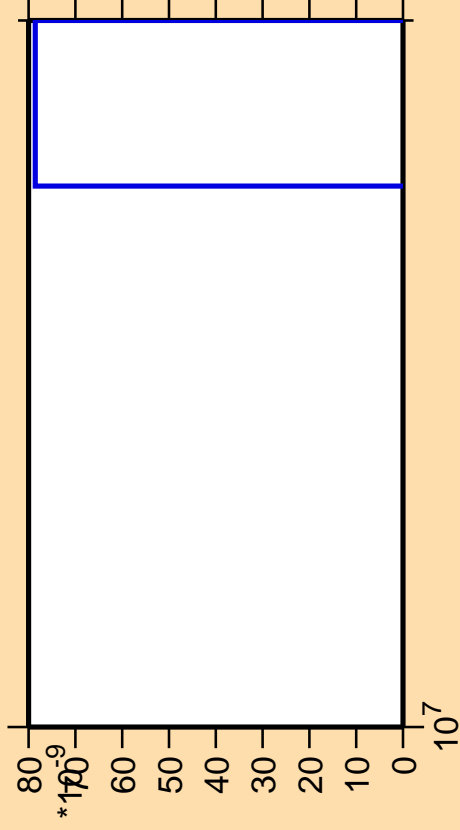
\Delta\sigma/\sigma vs. E for ^{189}\text{W} (mt 11)
