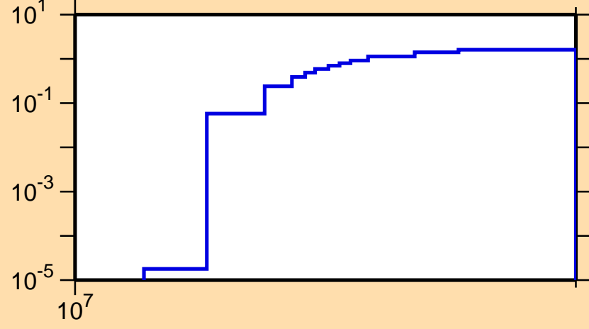
\sigma vs. E for ^{189}\text{W}(n,3n)
