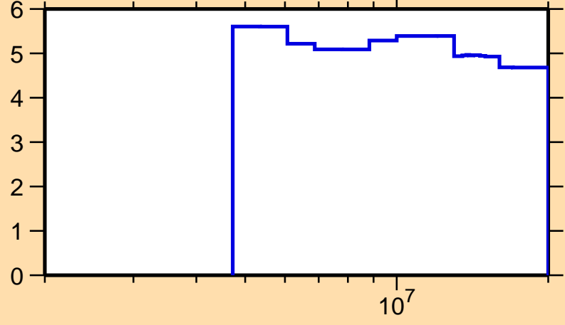
\Delta\sigma/\sigma vs. E for ^{189}\text{W}(n,\text{nonel.})
