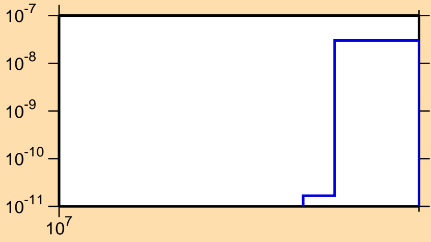
\sigma vs. E for ^{189}\text{W}(n,2np)
