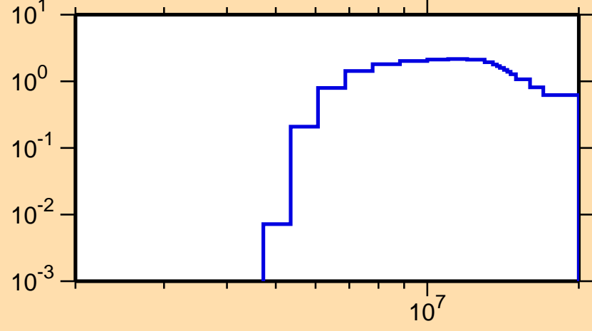
\sigma vs. E for ^{189}\text{W}(n,2n)
