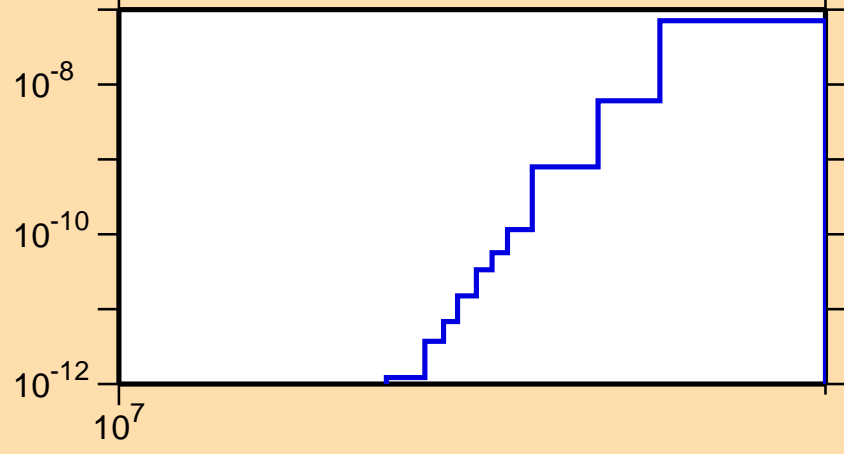
\sigma vs. E for ^{189}\text{W}(n,2n\alpha)
