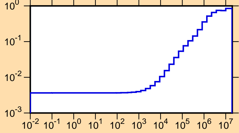
\mu vs. E for ^{189}\text{W}(\text{mt251})
