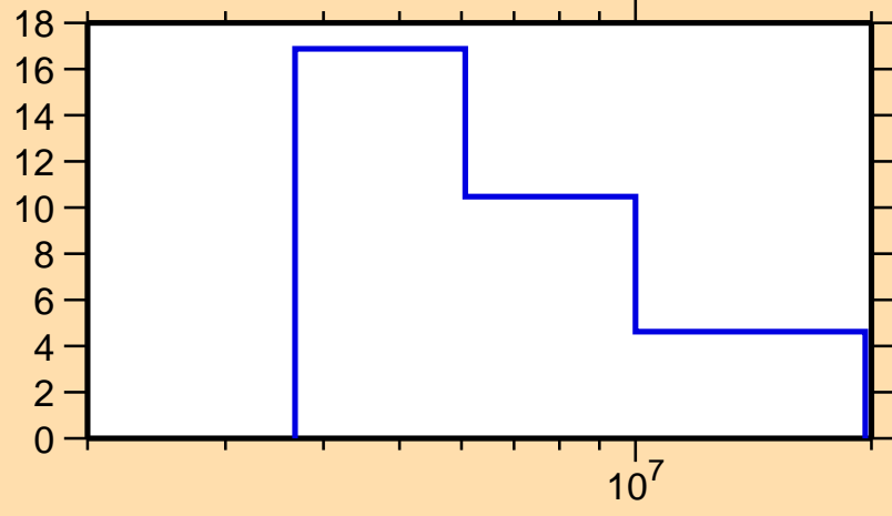
\Delta\sigma/\sigma vs. E for ^{189}\text{W}(n,el.)
