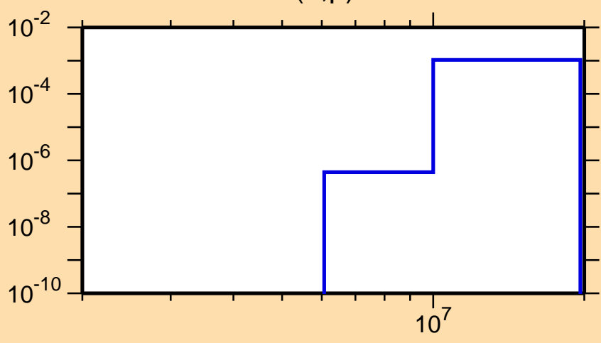
\sigma vs. E for ^{189}\text{W}(n,p)
