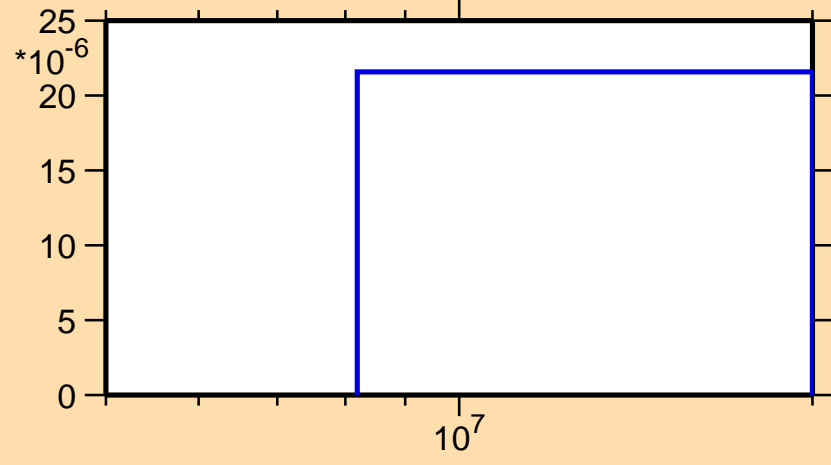
\sigma vs. E for ^{189}\text{W}(n,d)
