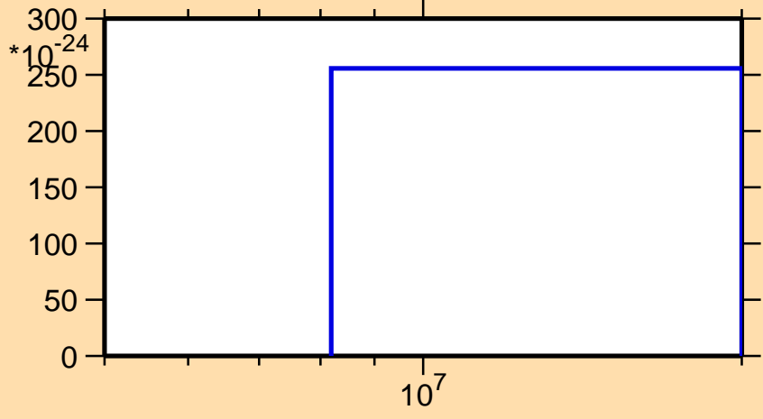
\sigma vs. E for ^{189}\text{W} (mt 11)
