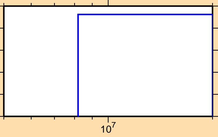
\sigma vs. E for ^{189}\text{W}(n,2n\alpha)
