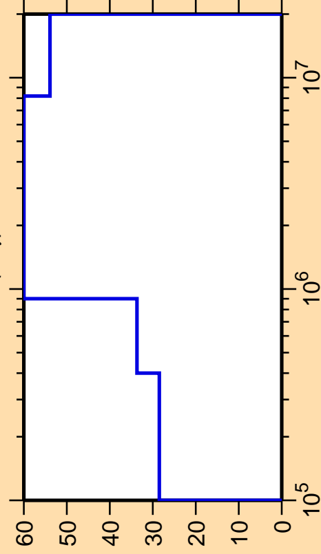
\Delta\sigma/\sigma vs. E for ^{189}\text{W}(n,\gamma)
