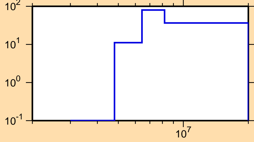
\Delta\sigma/\sigma vs. E for ^{189}\text{W}(n,p)
