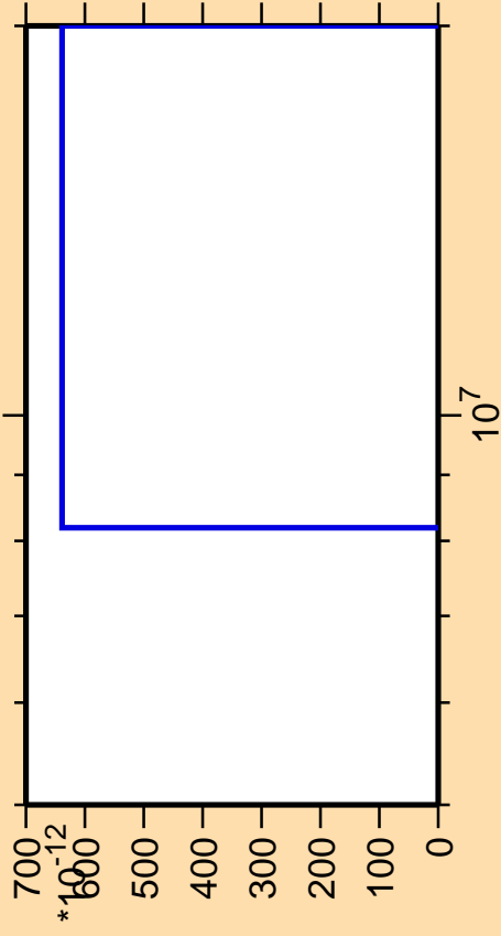
\Delta\sigma/\sigma vs. E for ^{189}\text{W} (mt 11)
