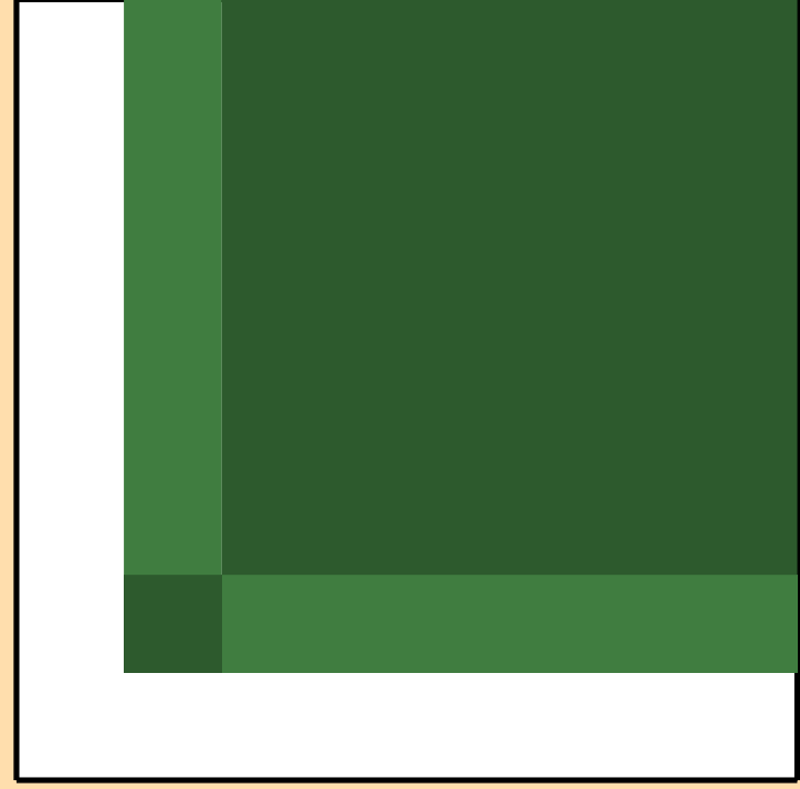
\sigma vs. E for ^{192}\text{W}(n,3n)
