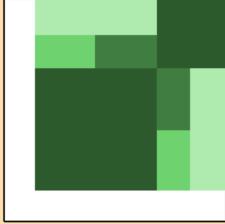
\sigma vs. E for ^{192}\text{W}(n,2n)
