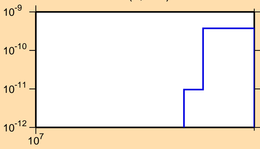
\sigma vs. E for ^{192}\text{W}(n,2n\alpha)
