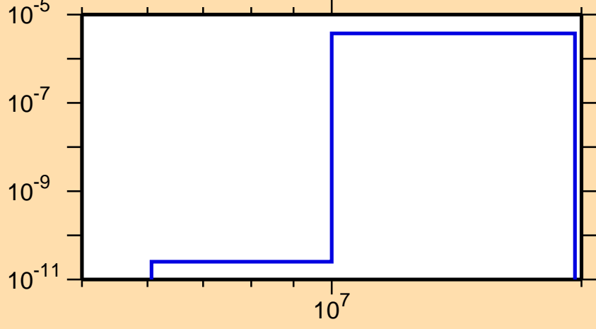
\sigma vs. E for ^{192}\text{W}(n,\alpha)
