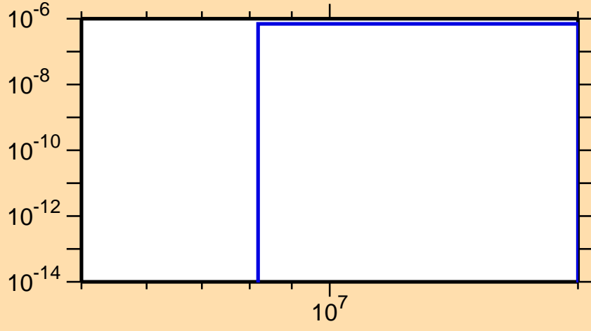
\sigma vs. E for ^{192}\text{W}(n,t)
