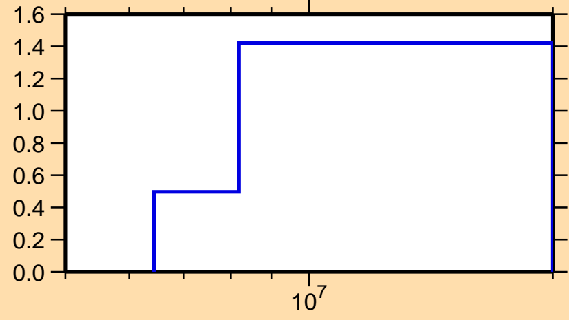
\sigma vs. E for ^{192}\text{W}(n,2n)
