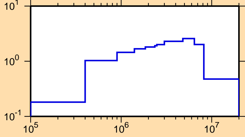
\sigma vs. E for ^{192}\text{W}(n,\text{inel.})
