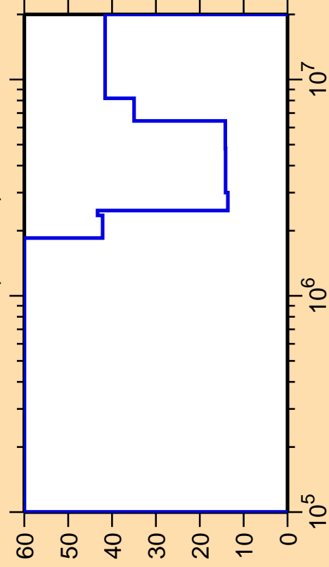
\Delta\sigma/\sigma vs. E for ^{192}\text{W}(n,\text{inel.})
