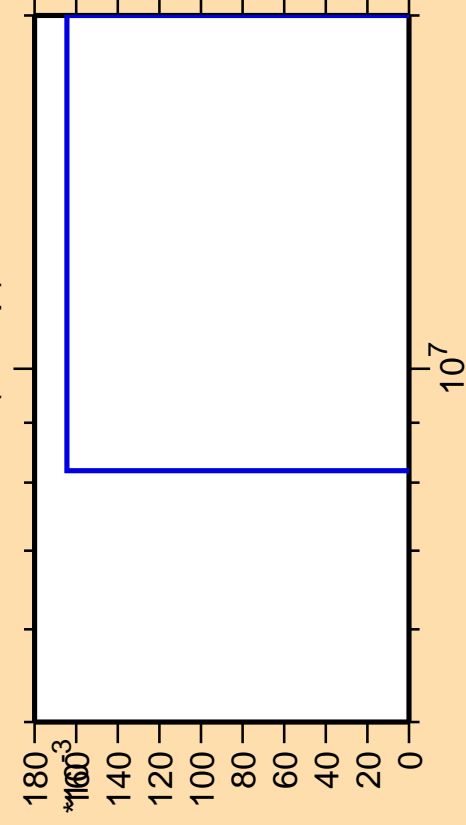
\Delta\sigma/\sigma vs. E for ^{192}\text{W}(n,2np)
