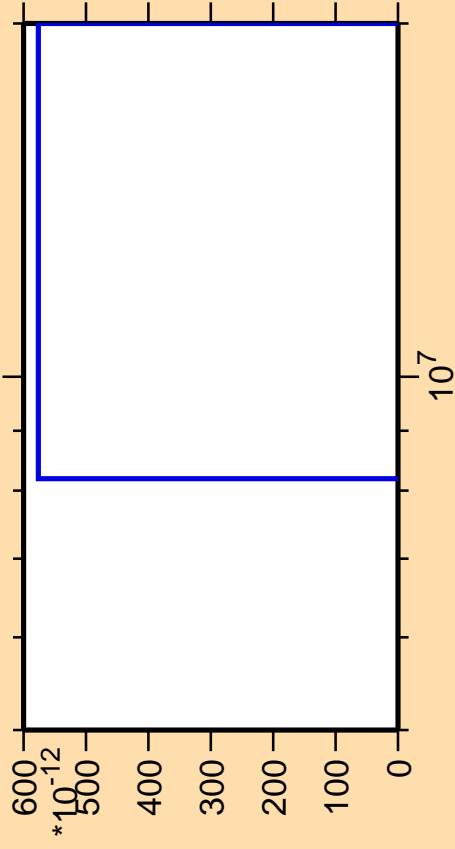
\Delta\sigma/\sigma vs. E for ^{192}\text{W} (mt 11)
