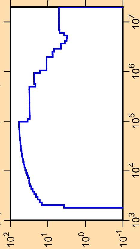
\Delta\mu/\mu vs. E for ^{194}\text{W}(\text{mt251})
