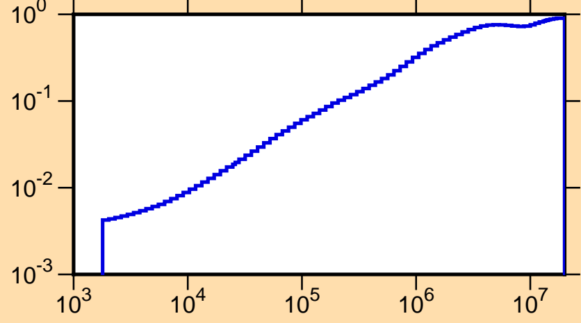
\mu vs. E for ^{194}\text{W}(\text{mt251})
