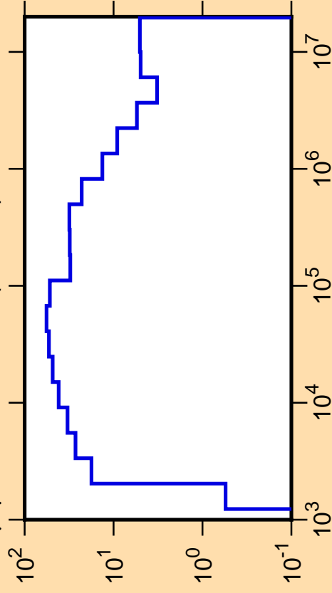
\Delta\mu/\mu vs. E for ^{194}\text{W}(\text{mt251})
