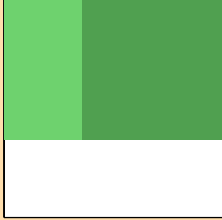
\Delta\sigma/\sigma vs. E for ^{194}\text{W}(n,\gamma)
