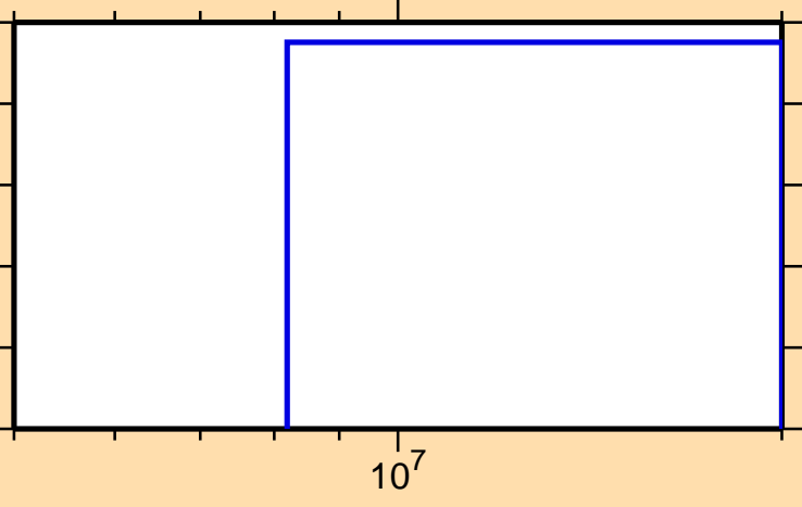
\sigma vs. E for ^{194}\text{W}(n,n\alpha)
