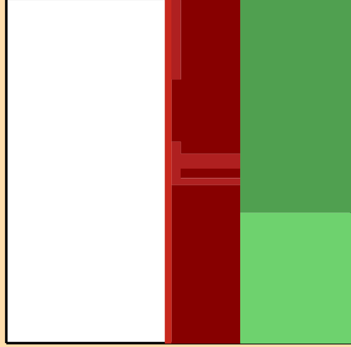
\Delta\sigma/\sigma vs. E for ^{112}\text{Xe}(n,2n)
