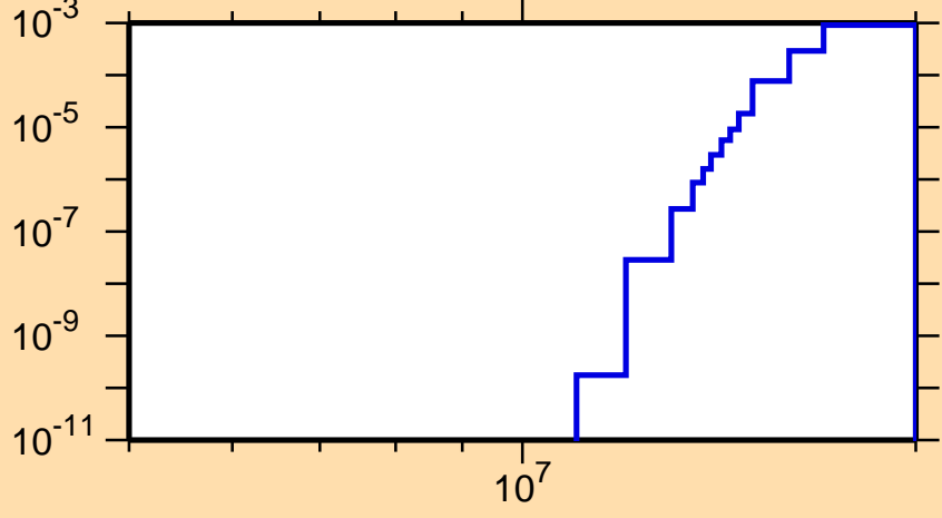
\sigma vs. E for ^{112}\text{Xe}(n,\text{pt})
