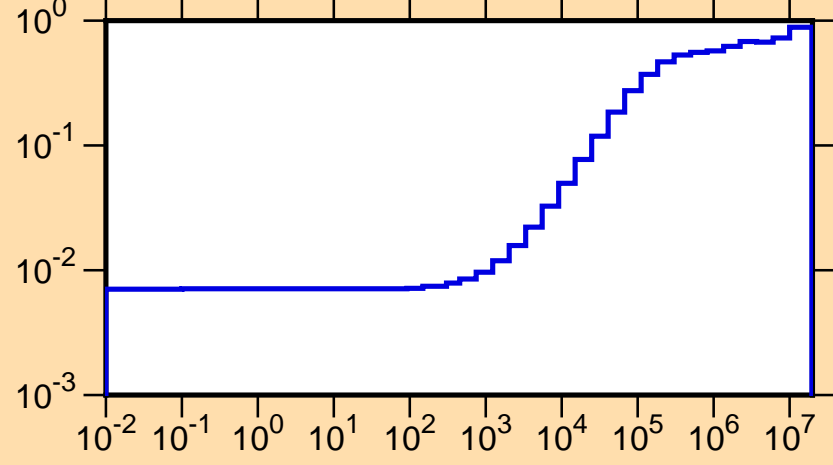
\mu vs. E for ^{112}\text{Xe}(\text{mt251})
