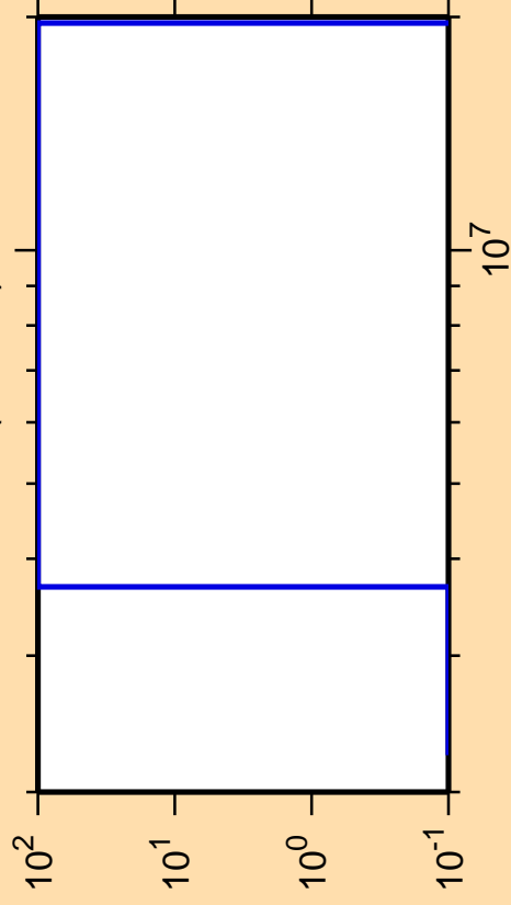
\Delta\sigma/\sigma vs. E for ^{112}\text{Xe}(\text{mt117})
