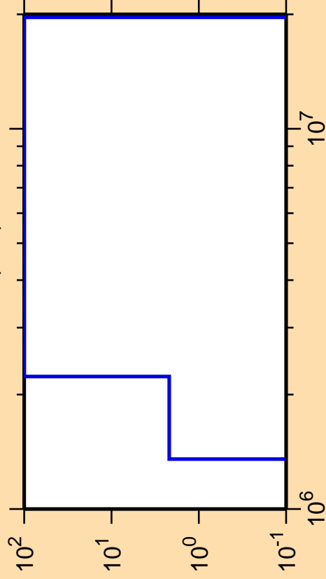
\Delta\sigma/\sigma vs. E for ^{112}\text{Xe}(n,d)
