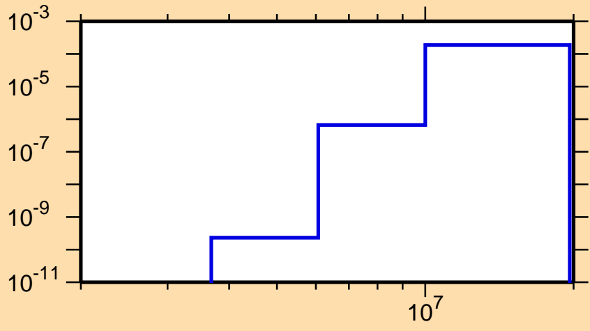
\sigma vs. E for ^{112}\text{Xe}(\text{mt117})
