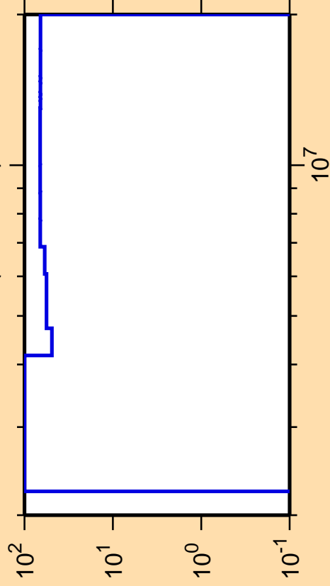
\Delta\sigma/\sigma vs. E for ^{113}\text{Xe}(n,\text{ncont.})
