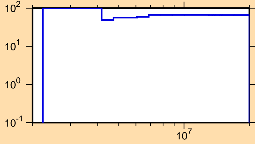
\Delta\sigma/\sigma vs. E for ^{113}\text{Xe}(n,ncont.)
