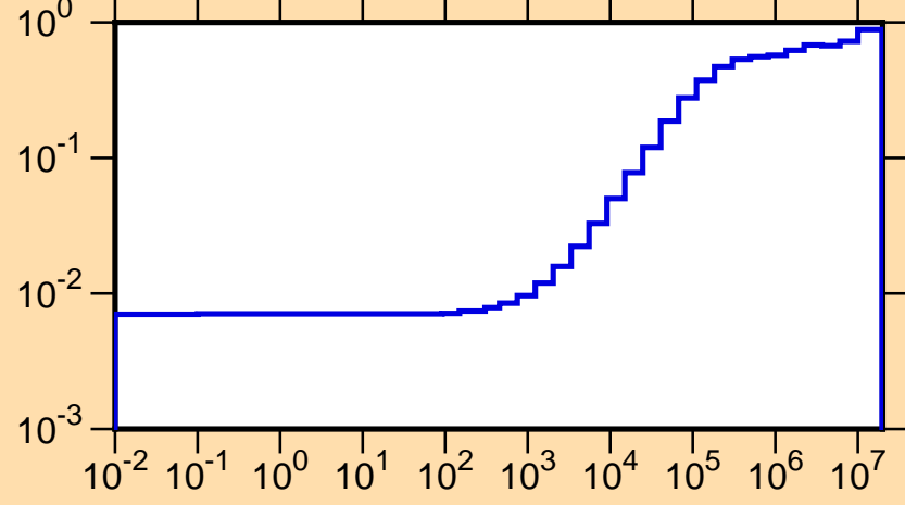
\mu vs. E for ^{113}\text{Xe}(\text{mt251})
