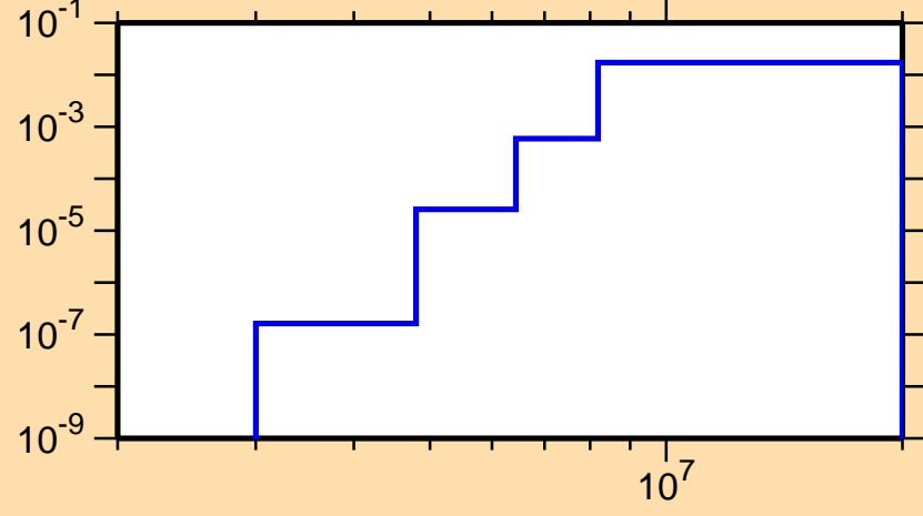
\sigma vs. E for ^{113}\text{Xe}(n,d)
