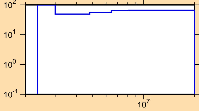
\Delta\sigma/\sigma vs. E for ^{113}\text{Xe}(n,n\text{cont.})
