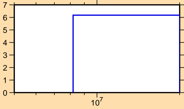
\Delta\sigma/\sigma vs. E for ^{113}\text{Xe}(n,\text{el.})
