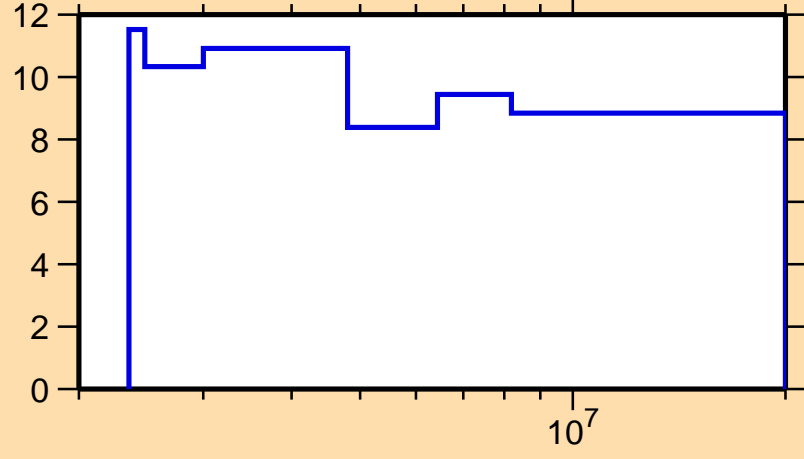
\Delta\sigma/\sigma vs. E for ^{113}\text{Xe}(n,\text{nonel.})
