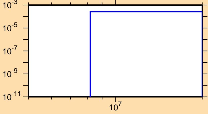
\sigma vs. E for ^{113}\text{Xe}(n,\text{pt})
