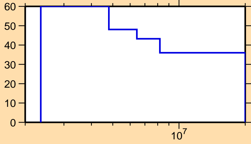
\Delta\sigma/\sigma vs. E for ^{113}\text{Xe}(n,\text{inel.})
