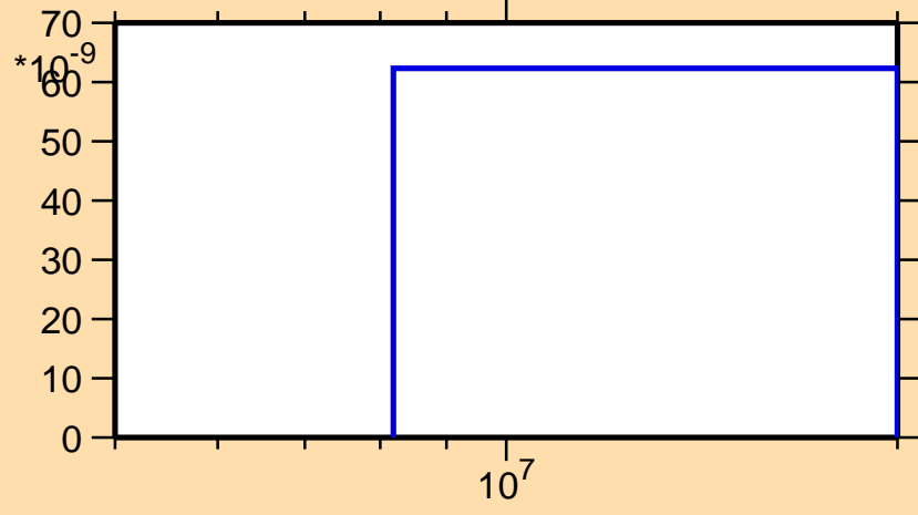
\sigma vs. E for ^{113}\text{Xe}(n,2n\alpha)
