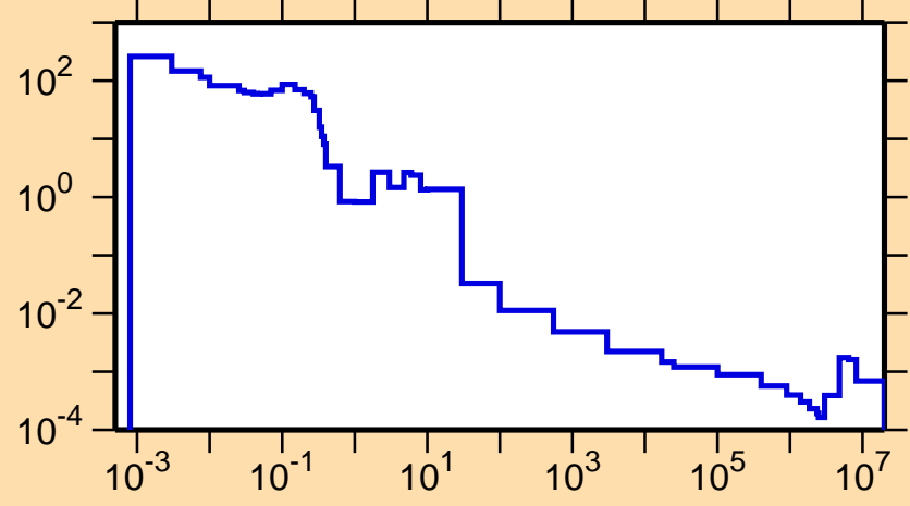
\sigma vs. E for ^{113}\text{Xe}(n,\gamma)
