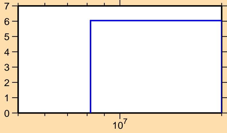
\Delta\sigma/\sigma vs. E for ^{113}\text{Xe}(n,\text{tot.})
