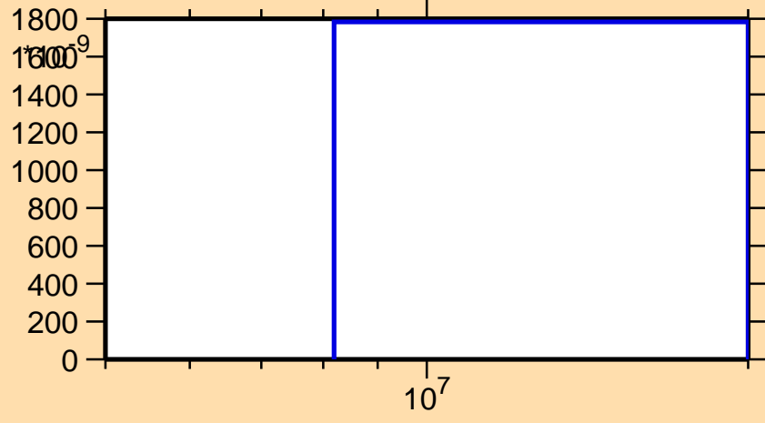
\sigma vs. E for ^{113}\text{Xe}(n,2np)
