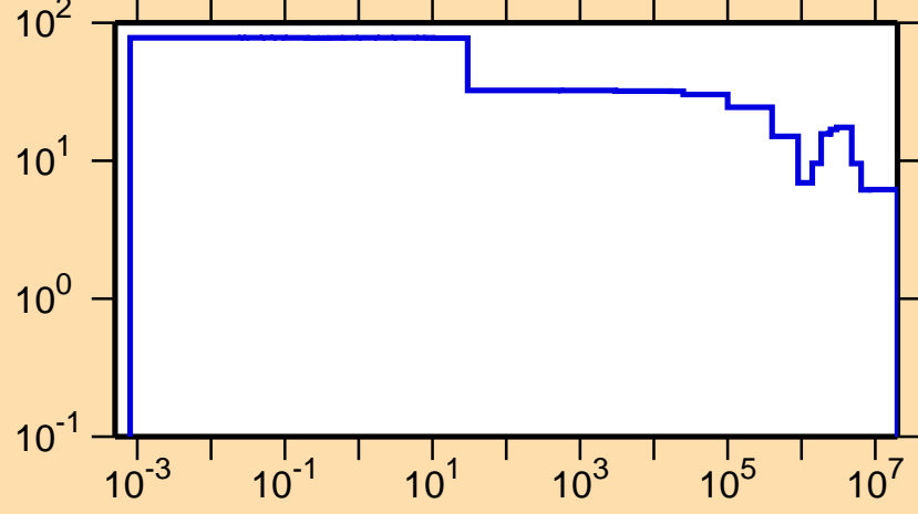
\Delta\sigma/\sigma vs. E for ^{113}\text{Xe}(n,\text{el.})
