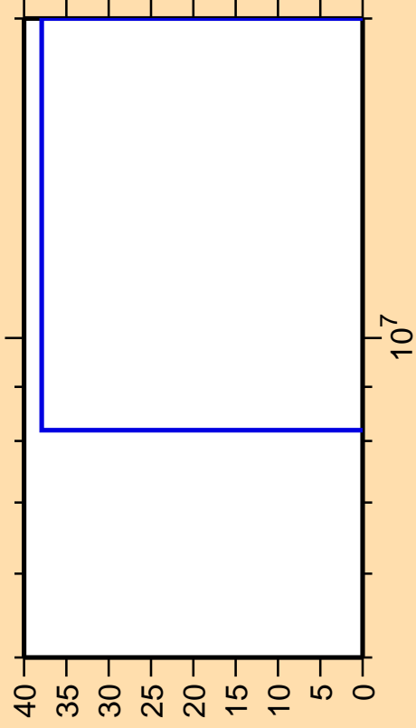
\Delta\sigma/\sigma vs. E for ^{113}\text{Xe}(n,n_1)
