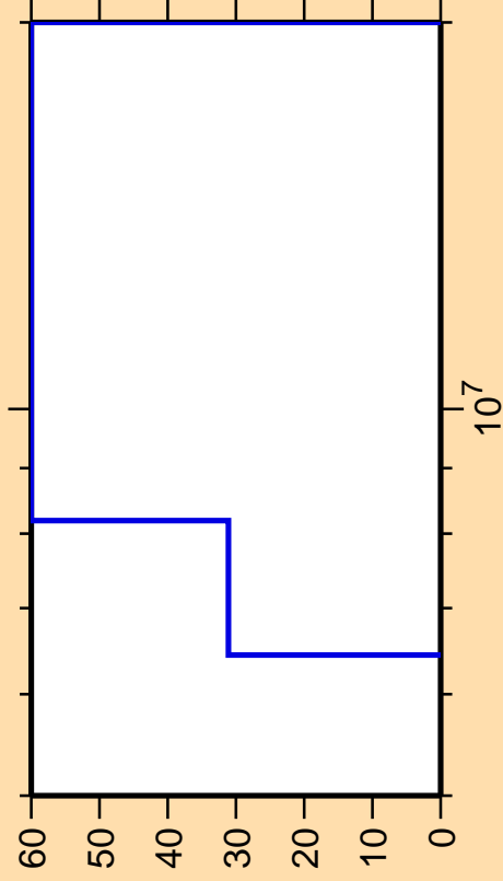
\Delta\sigma/\sigma vs. E for ^{113}\text{Xe}(\text{mt } 45)
