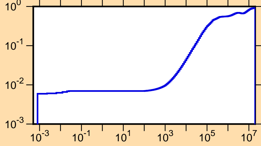
\mu vs. E for ^{115}\text{Xe}(\text{mt251})
