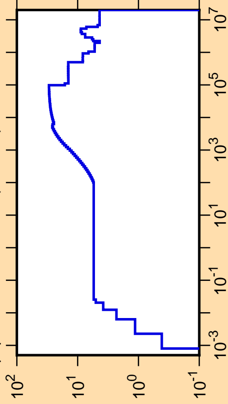
\Delta\mu/\mu vs. E for ^{115}\text{Xe}(\text{mt251})
