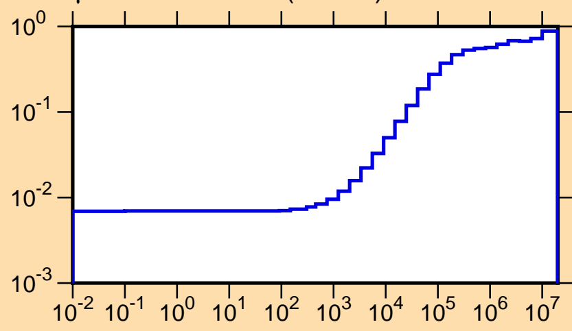
\mu vs. E for ^{115}\text{Xe}(\text{mt251})
