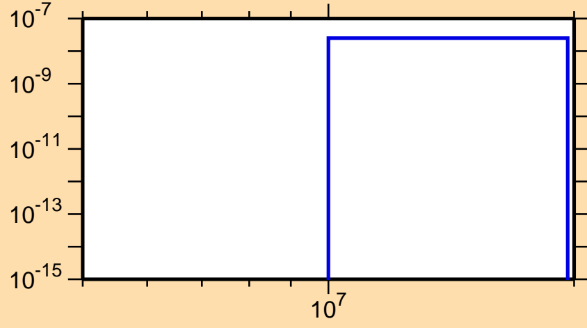
\sigma vs. E for ^{115}\text{Xe}(\text{mt } 34)
