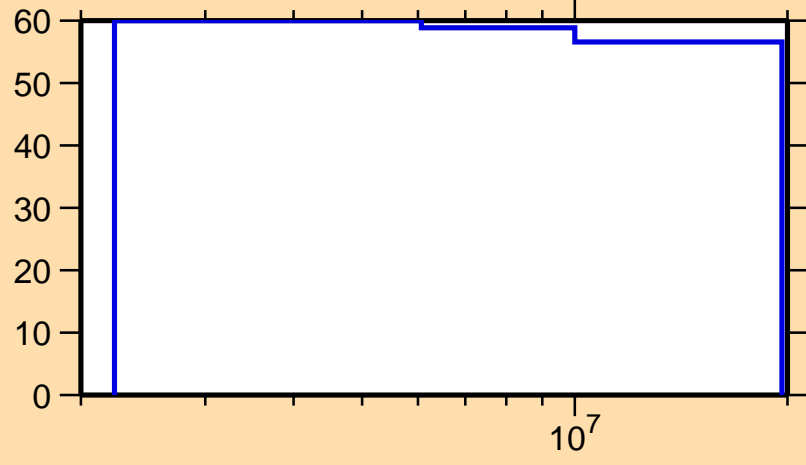
\Delta\sigma/\sigma vs. E for ^{115}\text{Xe}(n,ncont.)
