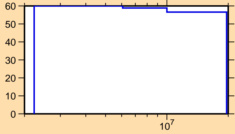
\Delta\sigma/\sigma vs. E for ^{115}\text{Xe}(n,n\text{cont.})
