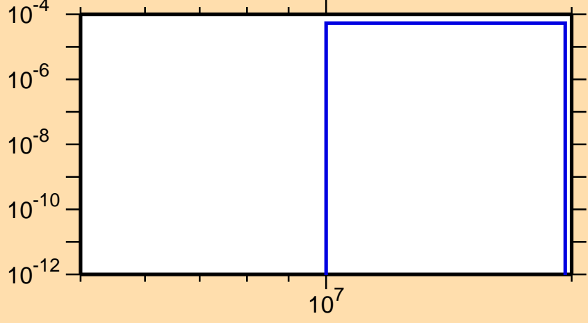
\sigma vs. E for ^{115}\text{Xe}(n,\text{pt})
