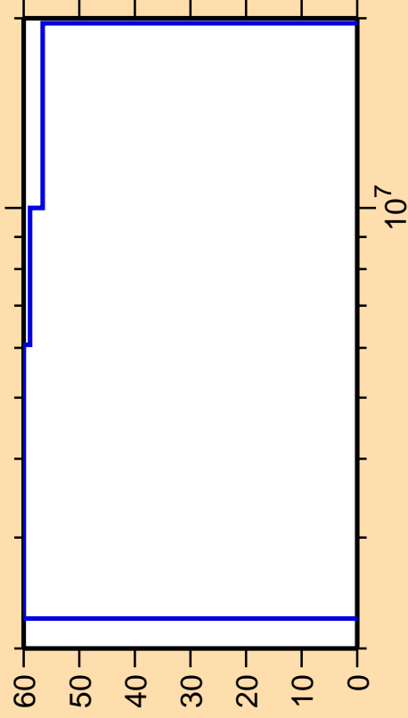
\Delta\sigma/\sigma vs. E for ^{115}\text{Xe}(n,\text{ncont.})
