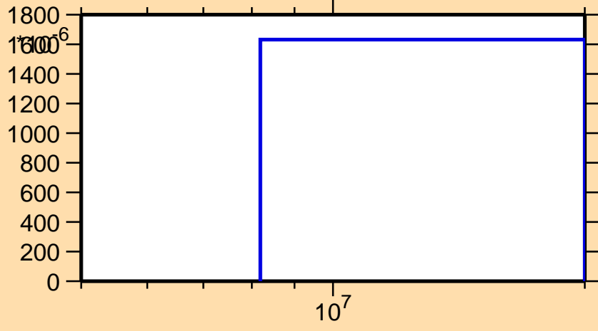
\sigma vs. E for ^{115}\text{Xe}(n,2n)
