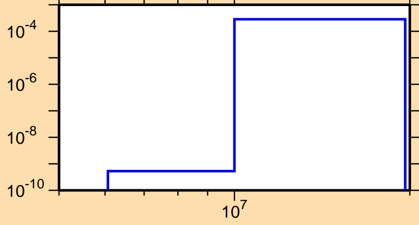
\sigma vs. E for ^{116}\text{Xe}(n,\text{pd})
