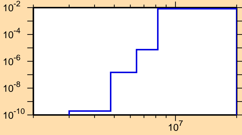
\sigma vs. E for ^{116}\text{Xe}(n,d)
