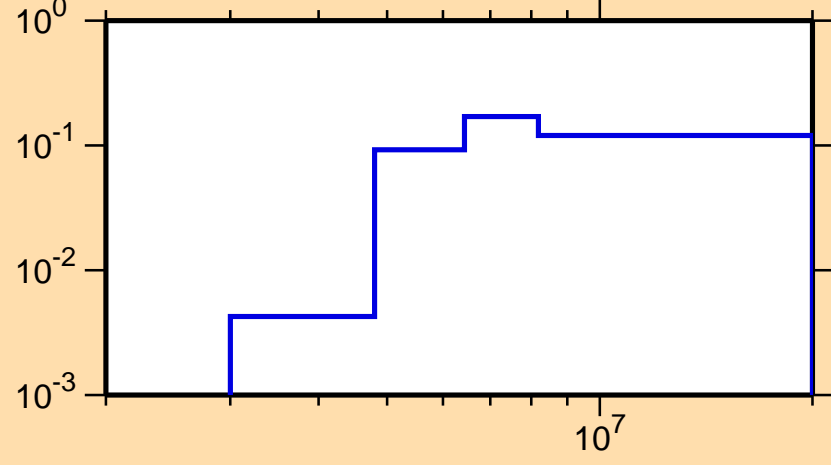
\sigma vs. E for ^{116}\text{Xe}(n,n\text{cont.})
