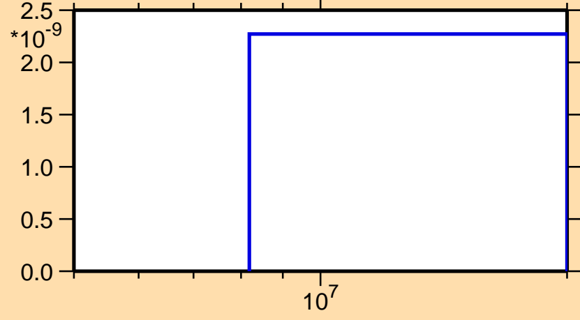
\sigma vs. E for ^{116}\text{Xe}(n,2n\alpha)
