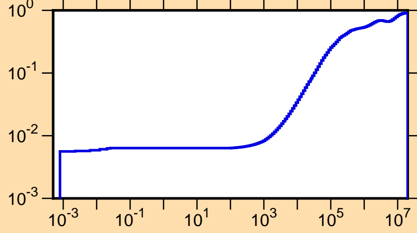
\mu vs. E for ^{121}\text{Xe}(\text{mt251})
