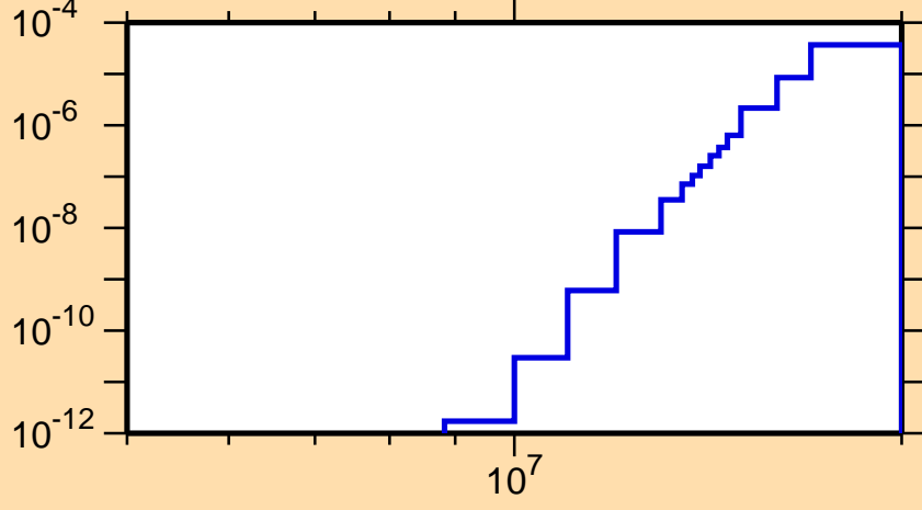
\sigma vs. E for ^{121}\text{Xe}(n,\text{He3})
