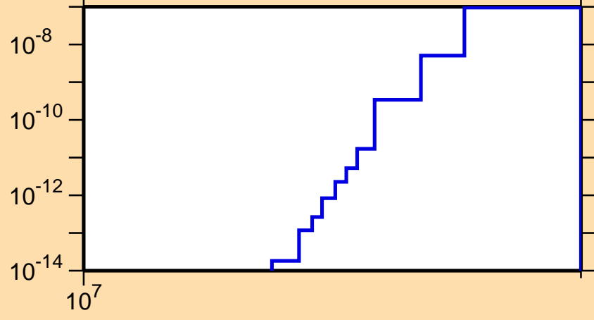
\sigma vs. E for ^{121}\text{Xe}(\text{mt } 45)
