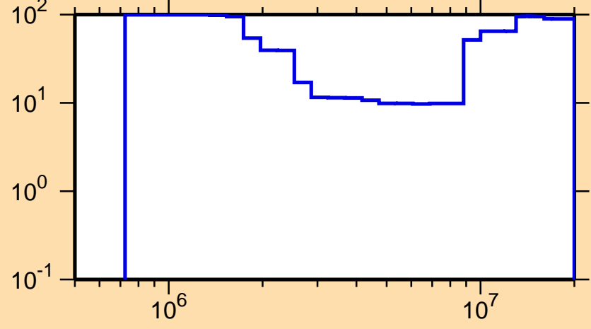
\Delta\sigma/\sigma vs. E for ^{121}\text{Xe}(n,n\text{cont.})
